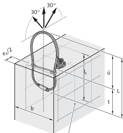
Fig. 2: Transverse installation
