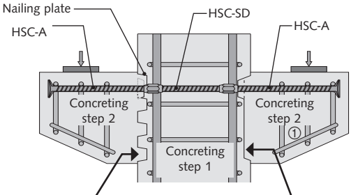
Variant 1: Indented joint in accordance with DIN EN 1992-1-1
