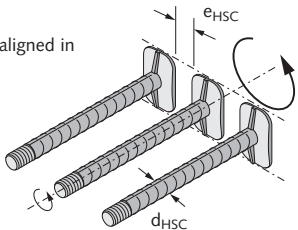
Min. distances to ensure installation (threaded bars)
