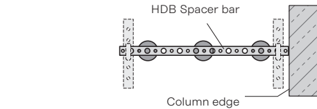
Figure 2b: Combination of 2 HDB Elements - plan view
