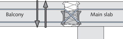
HIT-HP ZDX – High Performance 80 mm insulation thickness HIT-SP ZDX – Superior Performance 120 mm insulation thickness
