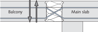
HIT-HP ZDX – High Performance 80 mm insulation thickness; without CSB HIT-SP ZDX – Superior Performance 120 mm insulation thickness; without CSB
