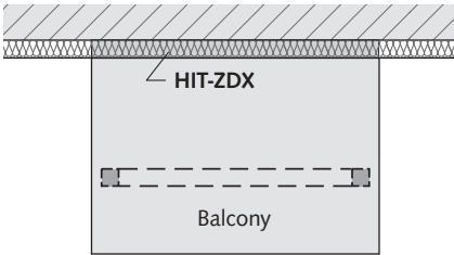
Application: Simply supported balcony on columns
