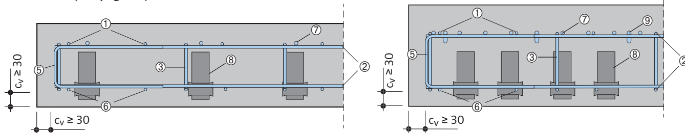
Section B-B, Example HIT-MVX
