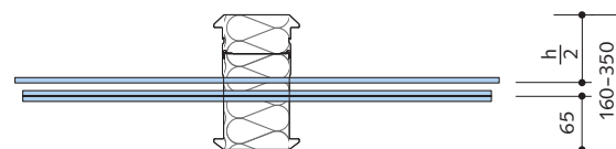
Top view HIT-HP HT3
