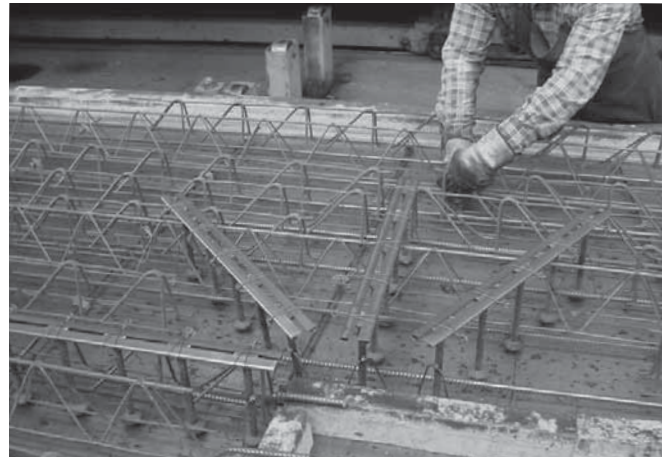
Production of precast elements using Halfen HDB-F Shear rails
