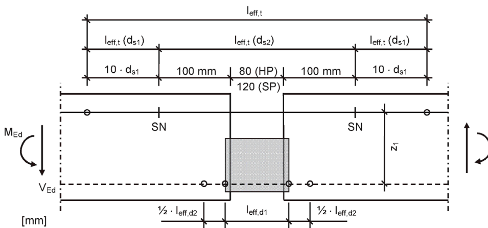
Figure 44: l_{\text{eff}} for stainless round steel S 460 and S 690 according to Annex A15
