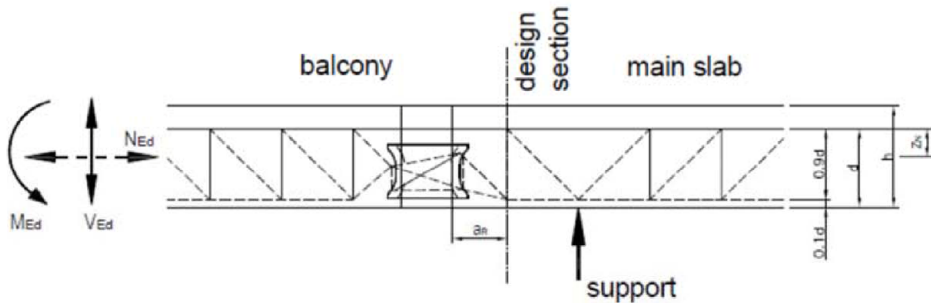
Figure 34: Strut-and-tie model and design section HIT-HP/SP MVX with compression shear bearing
