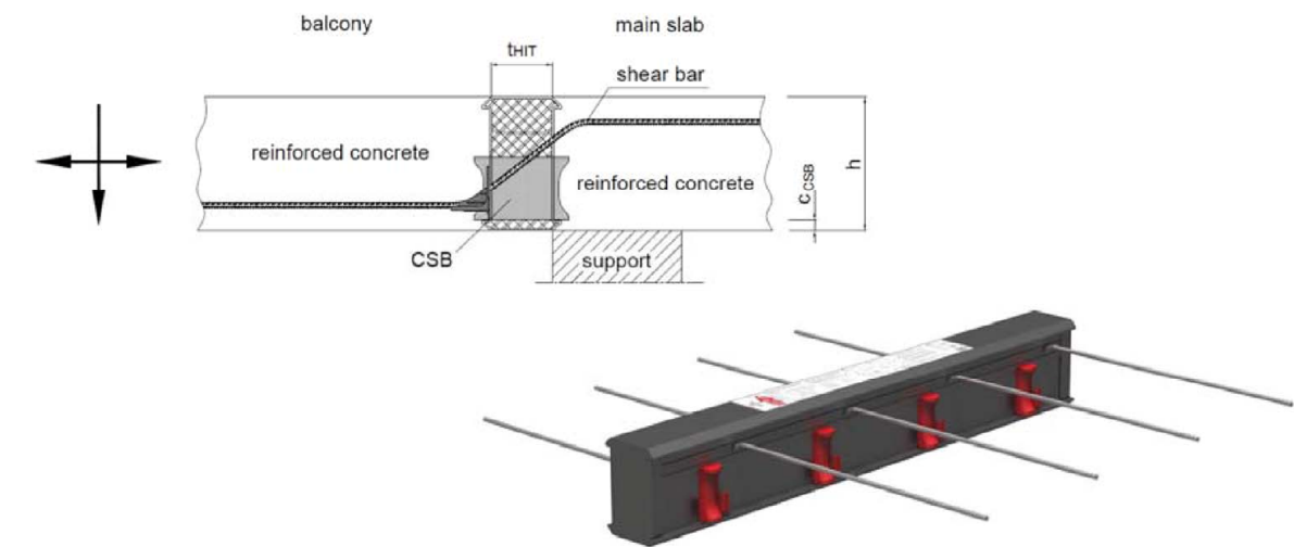
Figure 5: Halfen Insulated Connection HIT-HP/SP ZVX
