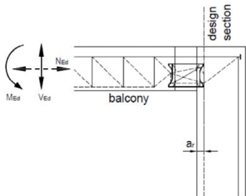
Figure 38: Strut-and-tie model HIT-HP/SP MVX-...-OU (wall connection)
