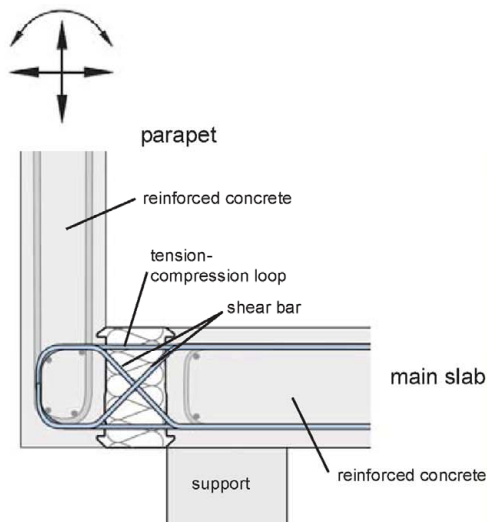
Figure 11: Halfen Insulated Connection HIT-HP/SP FT
