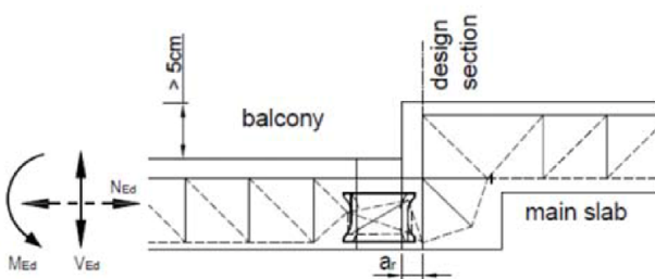
Figure 35: Strut-and-tie model HIT-HP/SP MVX-...-OD
